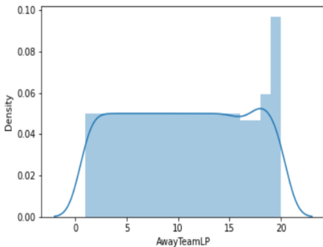
Fig 2 Density plot for AwayTeamLP
