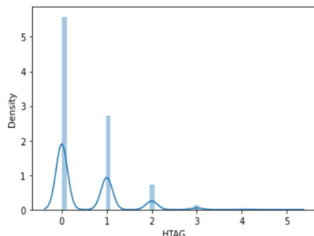
Fig 1 Density plots for HTAG
