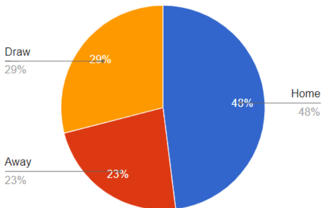
Fig 1 Classification of match wins from 2005 - 2020
